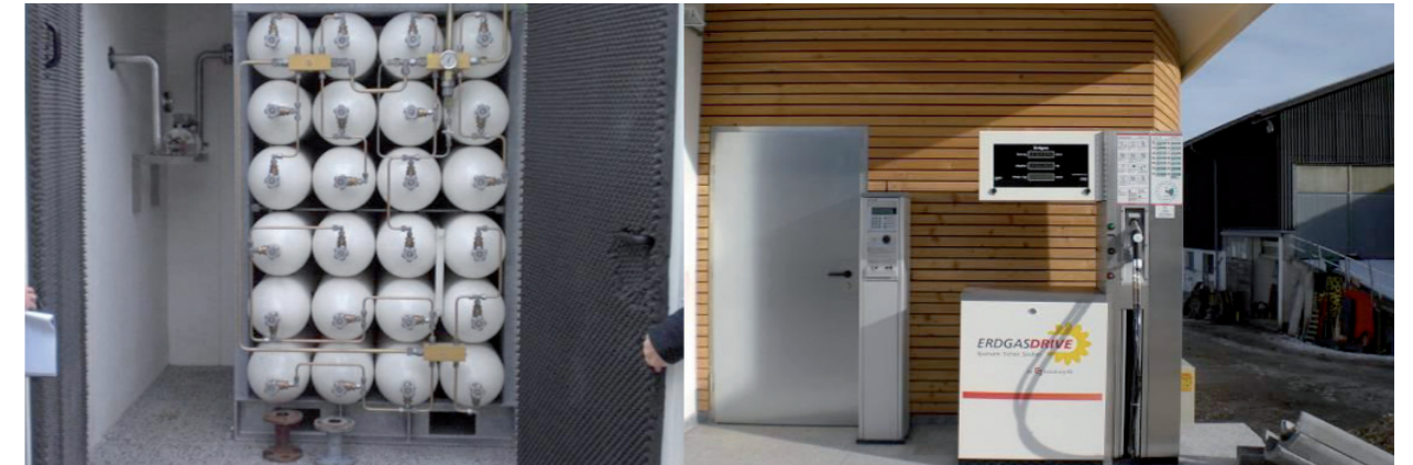
Photo 16: Storage cylinders for compressed biomethane and compressed biomethane dispenser on farm.
