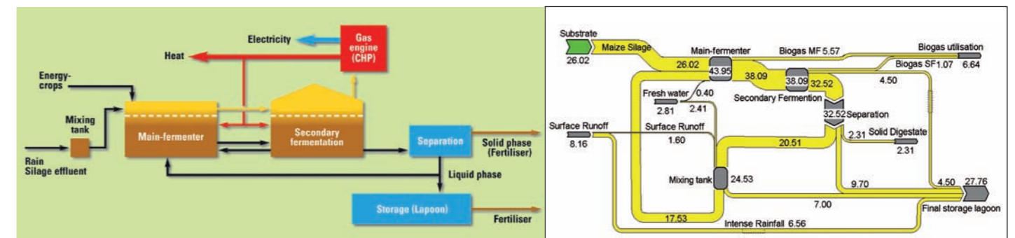
Figure 4: Flow chart of a two step crop digestion plant with 500 kW e electrical capacity. Solid crops (maize, grass) are used as substrates. Dilution of the substrate to less than 10% DS is achieved through recycling of liquid digestate and addition of leachate from the silage clamp
