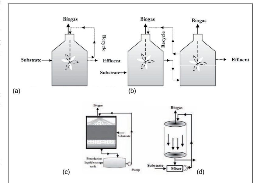
Figure 3: Reactor configurations (a) one step wet digestion (b) two step wet digestion (c) dry batch system (d) dry continuous system (Nizami and Murphy, 2010)
