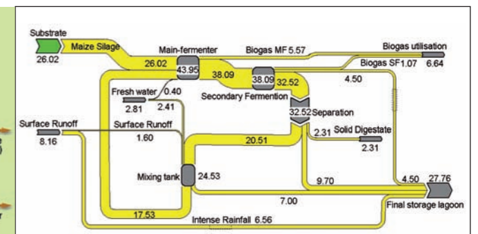
Figure 5: Mass flow diagram from a two-step crop digestion plant of 500 kW e electrical capacity. The plant uses liquid / solid separation of digestate and recycles the liquid digestate for substrate dilution. All data is given in tonnes / day. (Biogas MF represents biogas from the main digester; biogas SF indicates biogas from the second digester)
